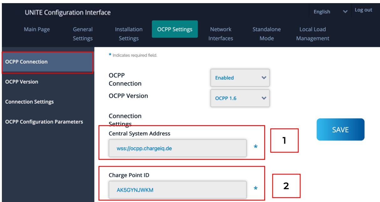
Abbildung 2-3: OCPP Connection
